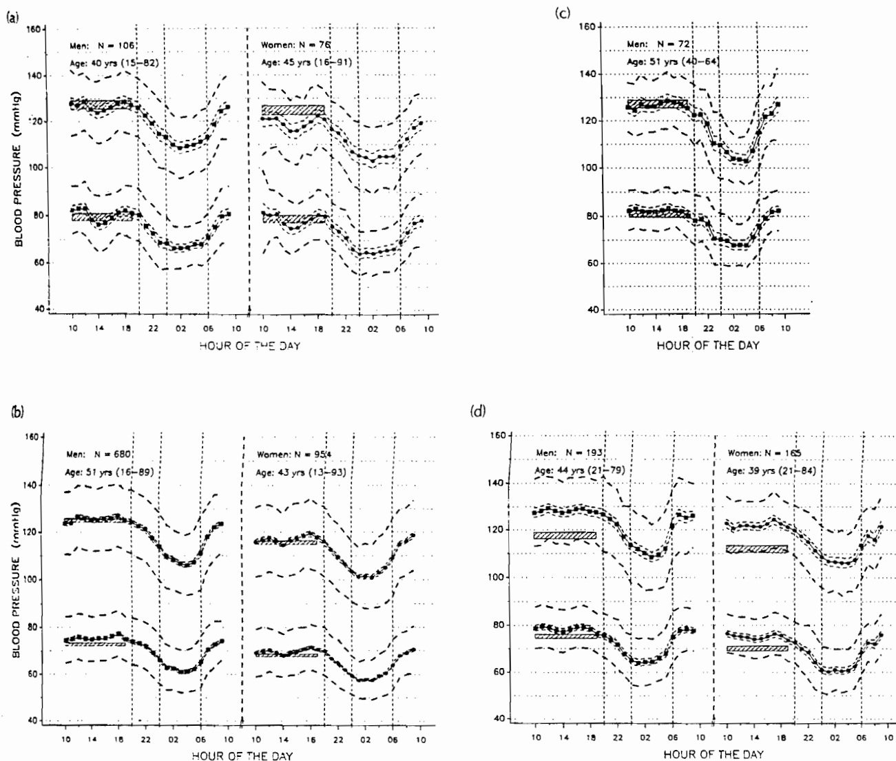
Fig. 2. Ambulatory blood pressure in normotensive subjects recruited in (a) Italy, (b) Japan, (c) Sweden and (d) the USA. Values are expressed as hourly means (with 95% confidence interval) \pm SD, for systolic and diastolic blood pressure in men (■) and women (●) separately. The shaded bands indicate the 95% confidence interval of the mean conventional blood pressure.
